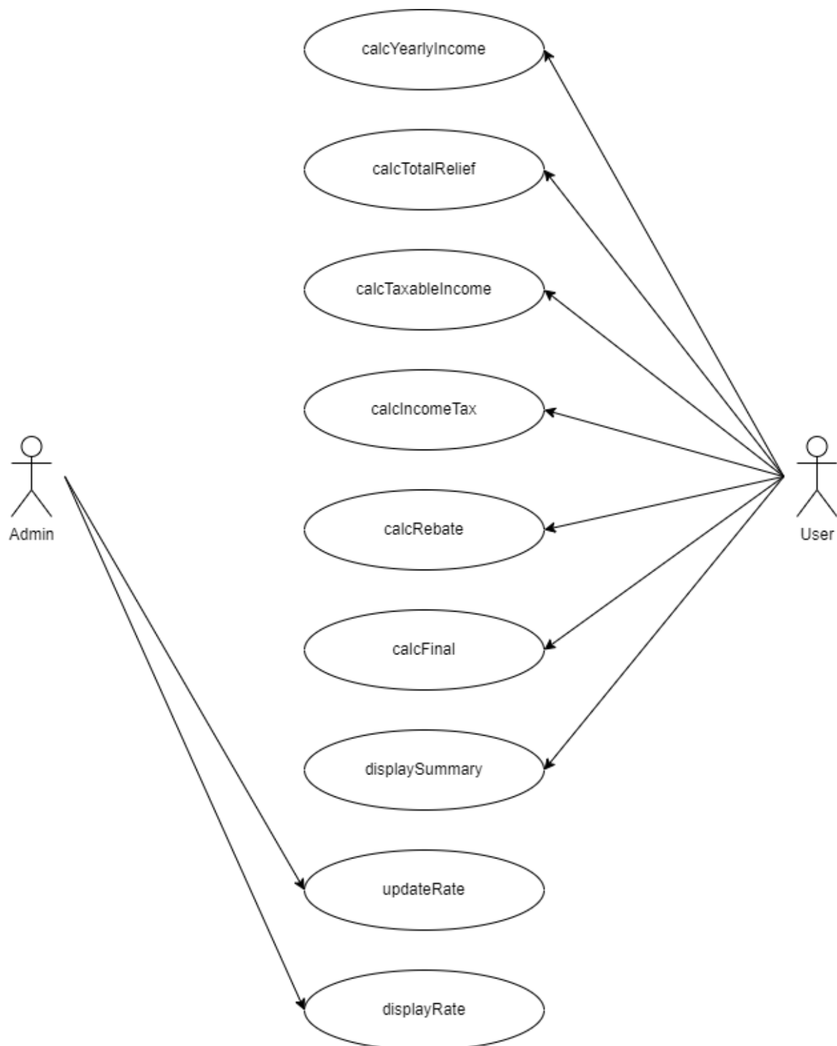
Figure 1 : Use Case Diagram for Tax Calculation System
